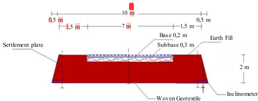
Fig.2 Embankment with Earth fill
