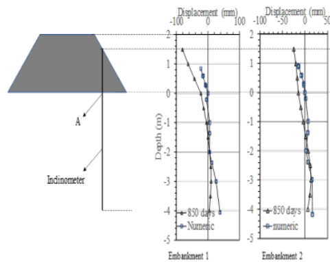
Fig.6 Horizontal Displacement Results
