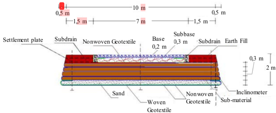
Fig.3 Embankment with Sub-material
