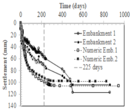
Fig.5 Time-Average Settlement Curves Obtained by Numeric and Settlement Plate Measurement
