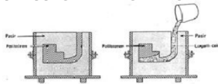
Gambar 1. Prinsip pengecoran evaporative
