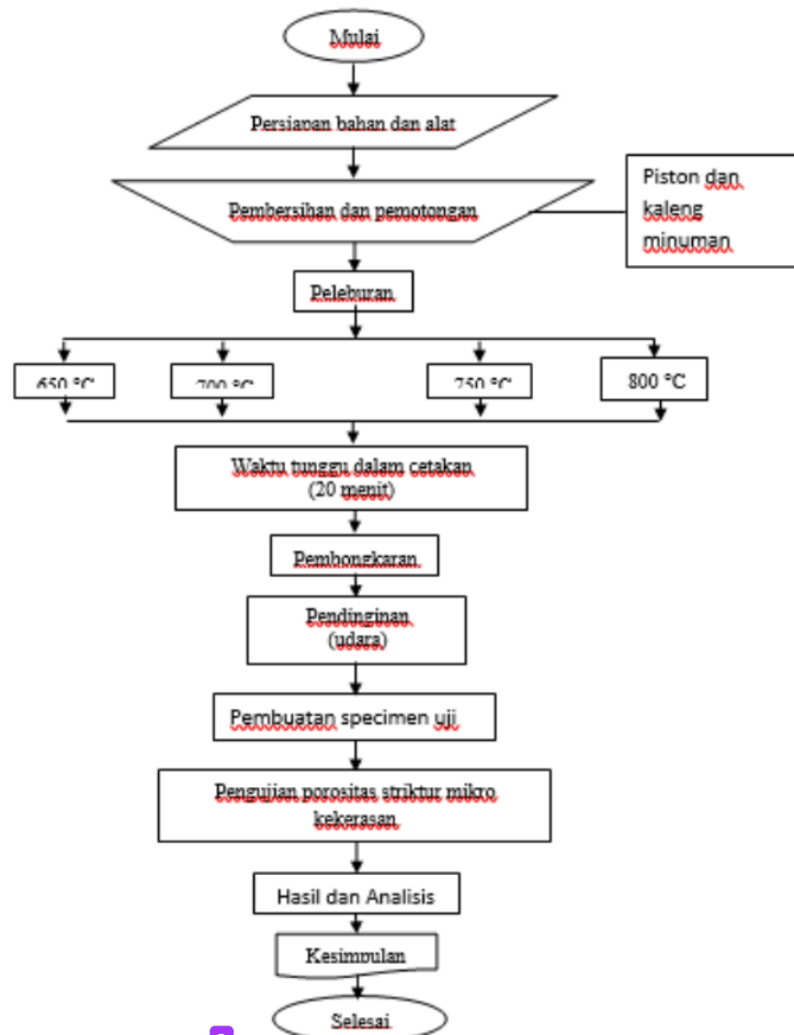
3 Gambar 1. Diagram Alir Penelitian
