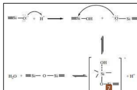
Figure 4. Reaction Mechanism of Silica Gel Formation
