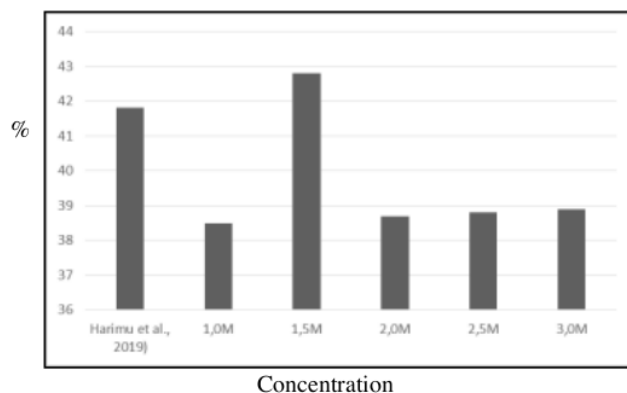
Figure 6. XRF Percentage of SiO 2 Siam Unus Rice Husk
