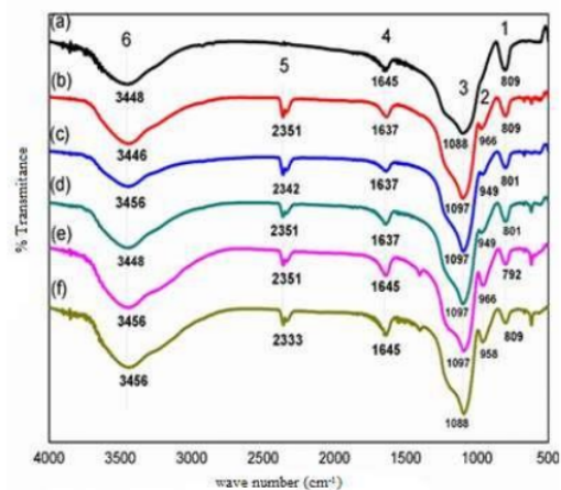
Figure 5. FTIR Spectra of (a) Siam Unus Rice Husk Ash, and silicate after extracted by NaOH variation concentration (b) 1.0 M, (c) 1.5 M, (d) 2.0 M (e) 2.5 M, (f) 3.0 M
