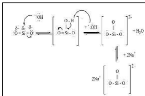
Figure 3. Reaction Mechanism of Sodium Silicate Formation (Mujiyanti et al., 2010)
