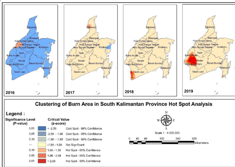
Figure 3. Clustering of Burned Area in South Kalimantan
