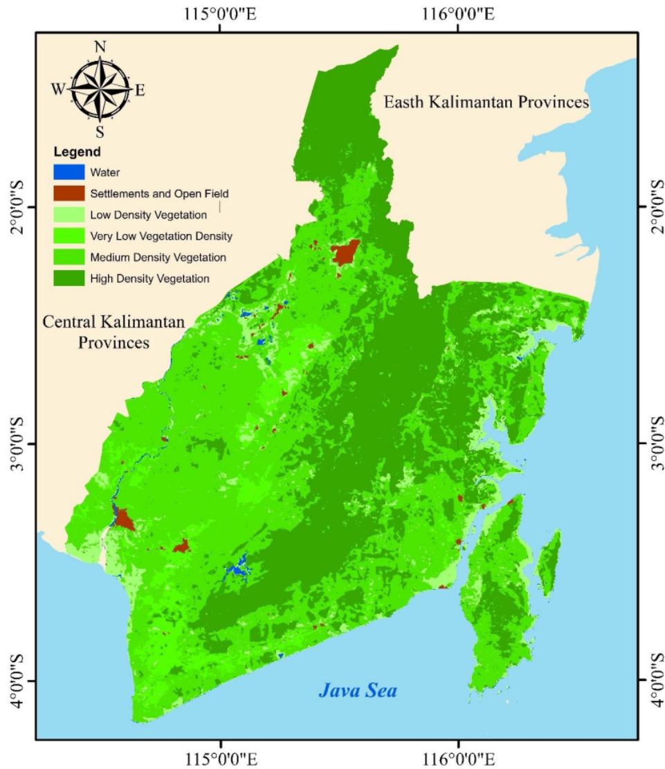
Figure 4. Land Cover in South Kalimantan Province (Source: MODIS Global Land Cover)
