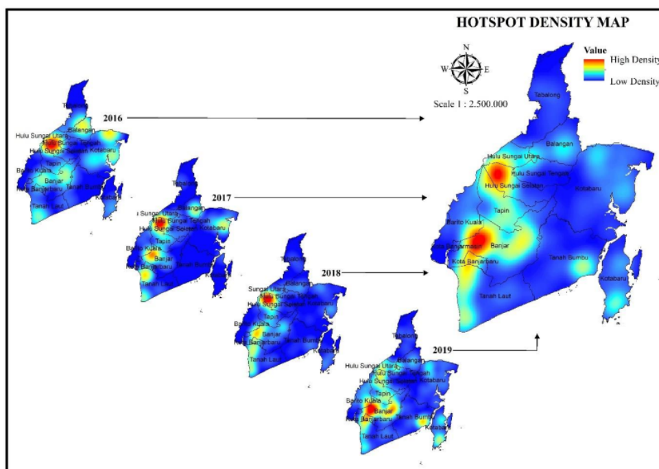
Figure 5. Map of Land Fire Density in South Kalimantan Province
