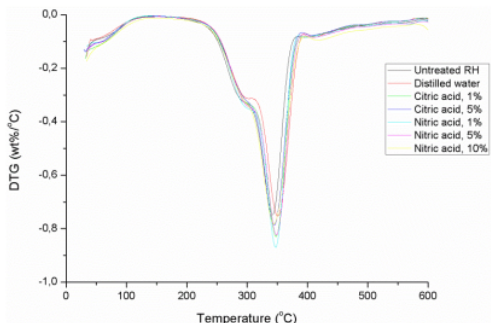
Figure 6. DTG plots of rice husk.
