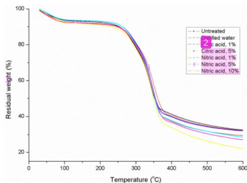
Figure 5. TGA plots of rice husk.
