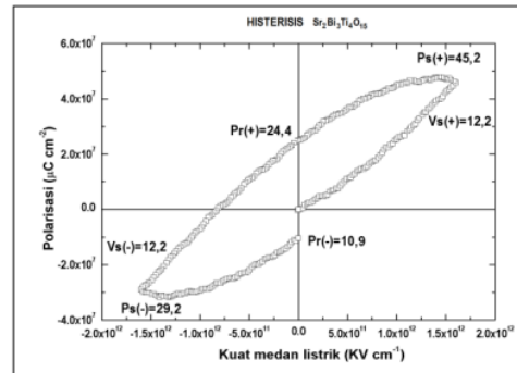
Gambar 11. Loop histerisis aurivillius \text{Sr}_2\text{Bi}_3\text{Ti}_4\text{O}_{15} (Mikrianto et al. , 2016)
