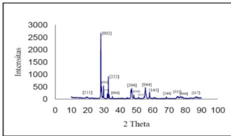
Gambar 8. Difraktogram aurivillius \text{Sr}_3\text{Bi}_3\text{Ti}_6\text{O}_{21} sintesis suhu 200^\circ\text{C} selama 72 jam (Mikrianto et al. , 2016).
