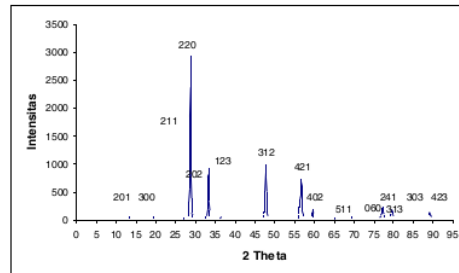
Gambar 2. Difraktogram aurivillius \text{SrBi}_3\text{Ti}_3\text{O}_{12} sintesis suhu 200 °C selama 72 jam (Mikrianto et al. , 2016).
