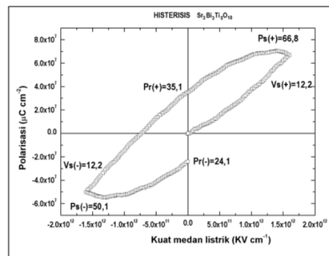
Gambar 12. Loop histerisis aurivillius \text{Sr}_3\text{Bi}_3\text{Ti}_5\text{O}_{18} (Mikrianto et al. , 2016)
