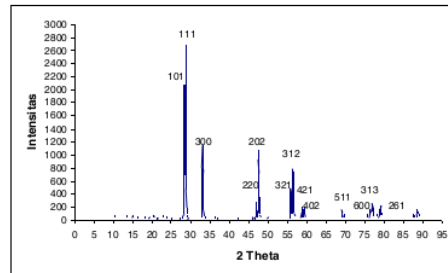
Gambar 6. Difraktogram aurivillius \text{Sr}_3\text{Bi}_3\text{Ti}_5\text{O}_{18} sintesis suhu 200 °C selama 72 jam (Mikrianto et al. , 2016).
