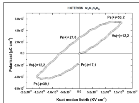
Gambar 13. Loop histerisis aurivillius \text{Sr}_3\text{Bi}_3\text{Ti}_6\text{O}_{21} (Mikrianto et al. , 2016).
