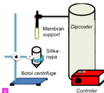
2 Gambar 1. Rangkaian Alat Proses Dipcoating
