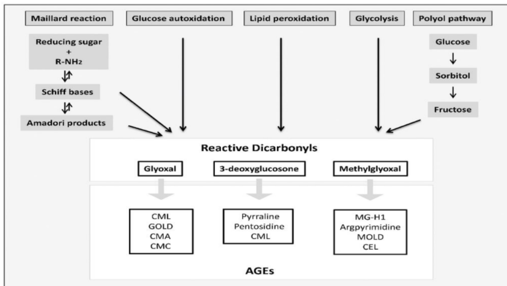
Figure 1. Formation of AGEs (Nowotny, 2015)
