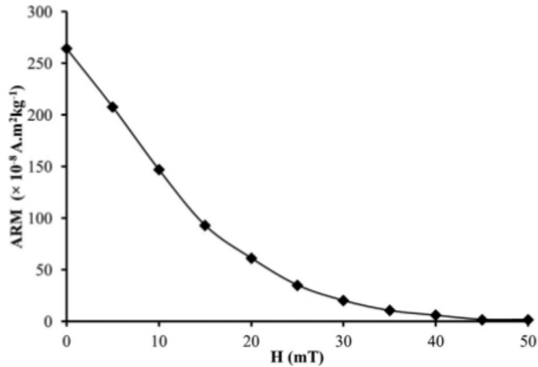
Fig. 1. ARM decay curve for typical bulk surface sediment sample (modified after [1]).
