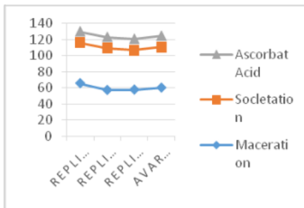
Figure 1. Curve of antioxidant activity test result by DPPH method.
